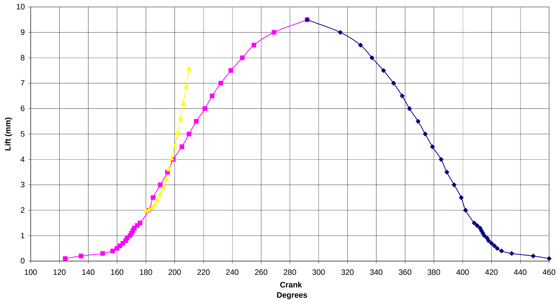
K100 Cam Profile
