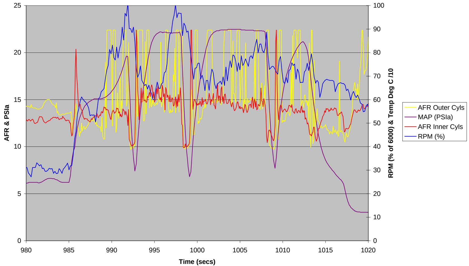
Dual Wideband Datalog - 05/07/09 - Siamesed Code - Turbo
