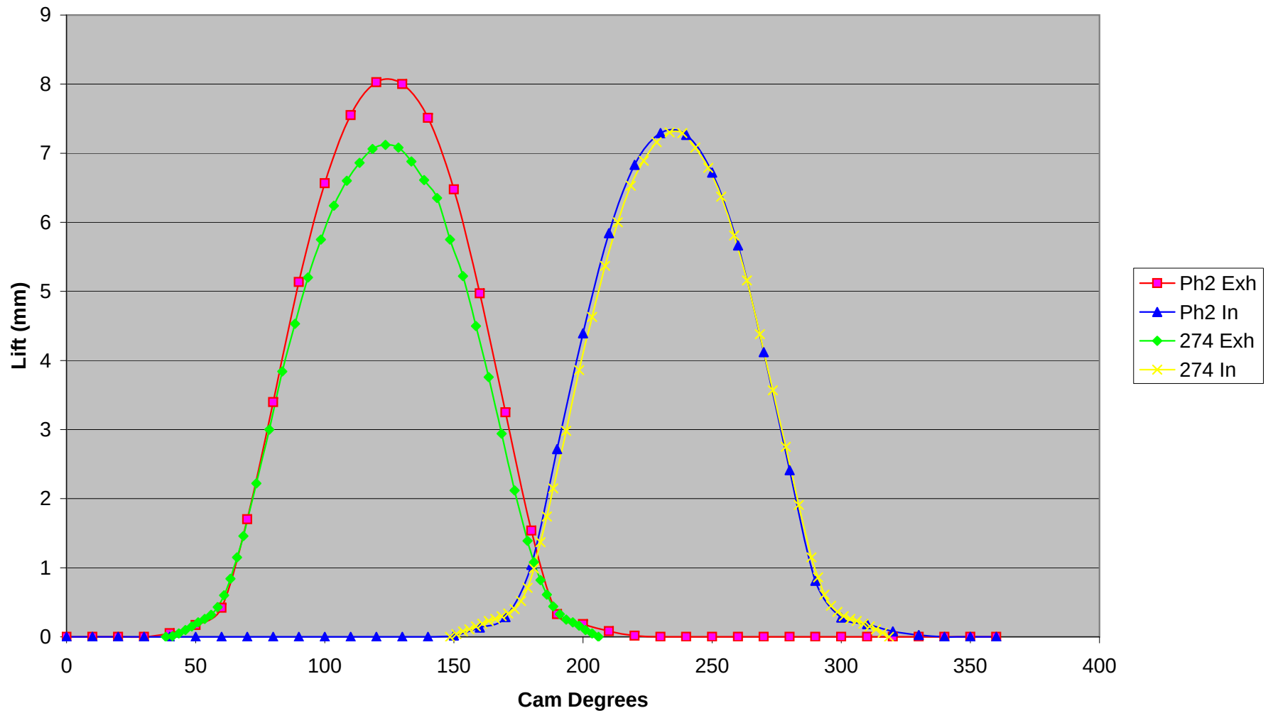
Cam Measurements
