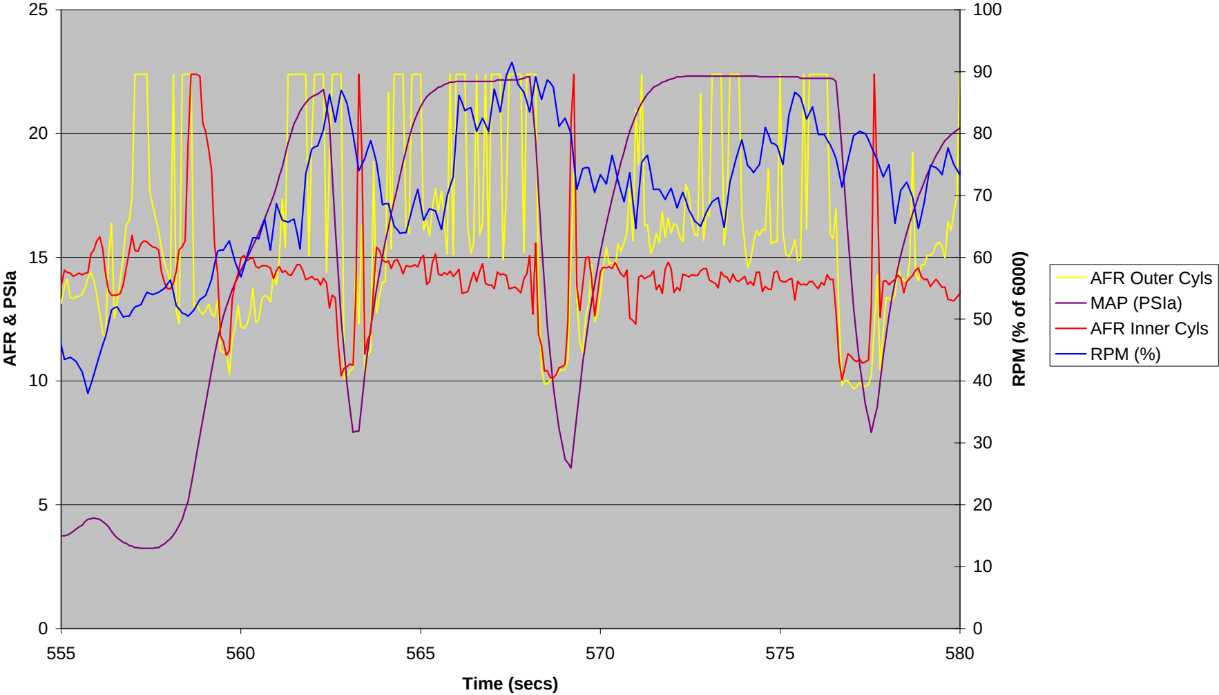
Dual Wideband Datalog - 05/07/09 - Siamesed Code - Turbo
